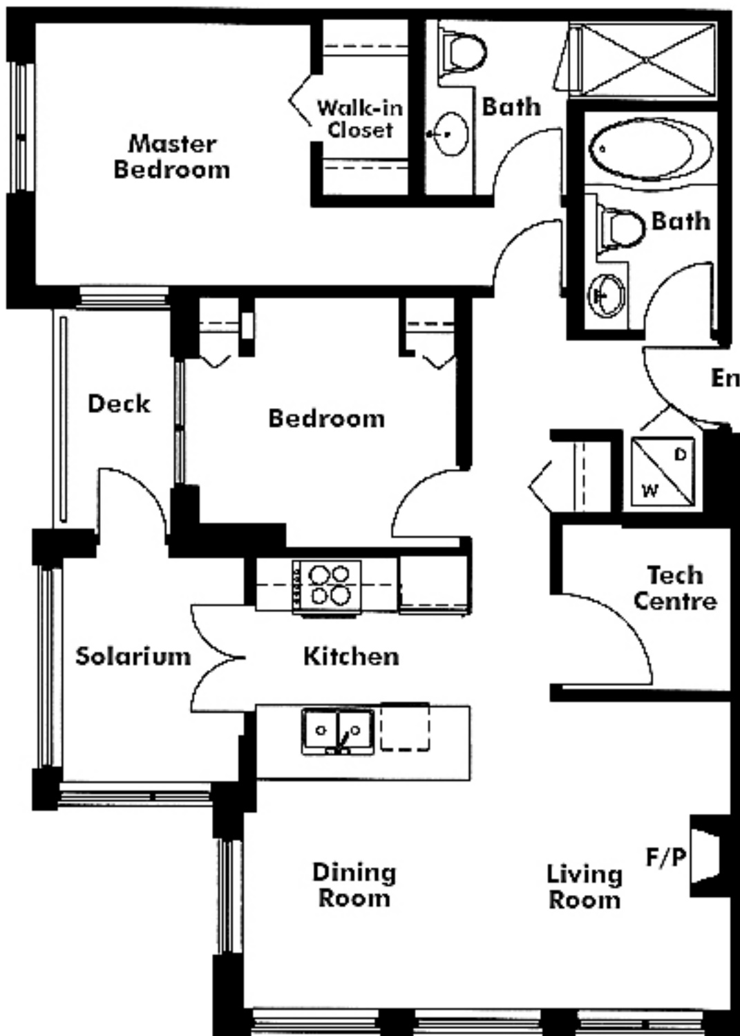
The Bentley 1001 Homer 5th - 23rd Floor (There is one 1,000 sq. ft. unit)
