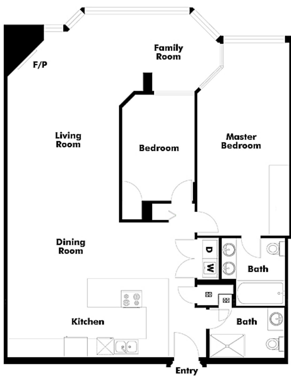
Harbour Cove 3 1490 Pennyfarthing 4th Floor
